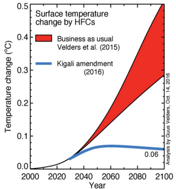
Estimated Climate Impact of Kigali Amendment by 2100
